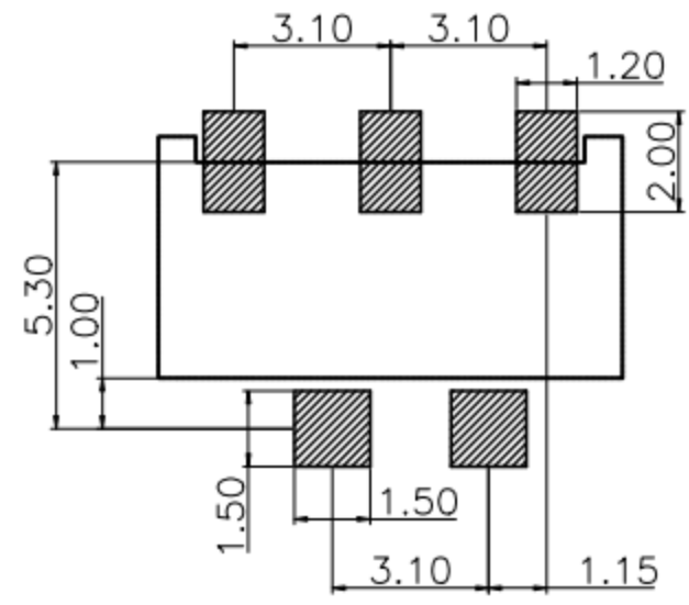
PCB Layout
